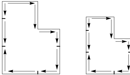
FIGURE 2. Markings by Grünbaum-Shephard in [9]
