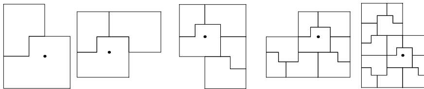
FIGURE 9. Inflation subdivision
