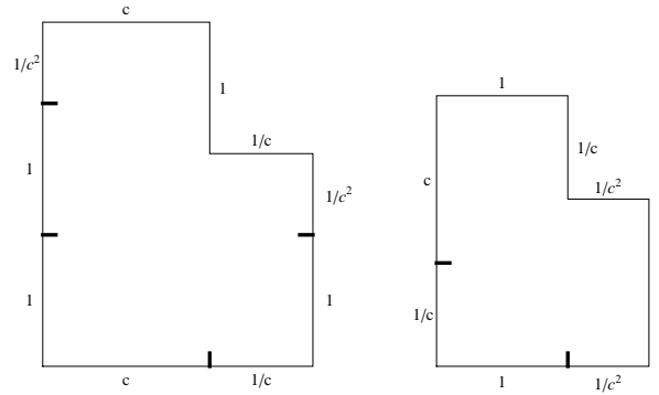
FIGURE 1. Similar Ammann tiles A and B
