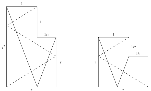
FIGURE 12. Ammann Bars
